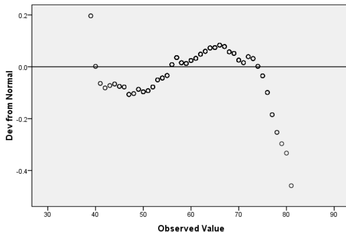
Detrended Normal Q-Q Plot of Penganbilen Keputusan
