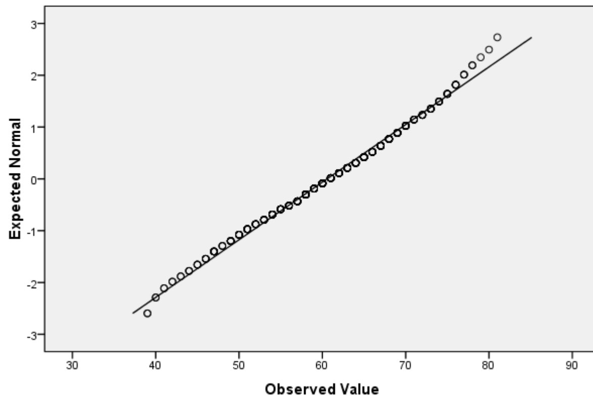
Normal Q-Q Plot of Pengambilan Keputusan
