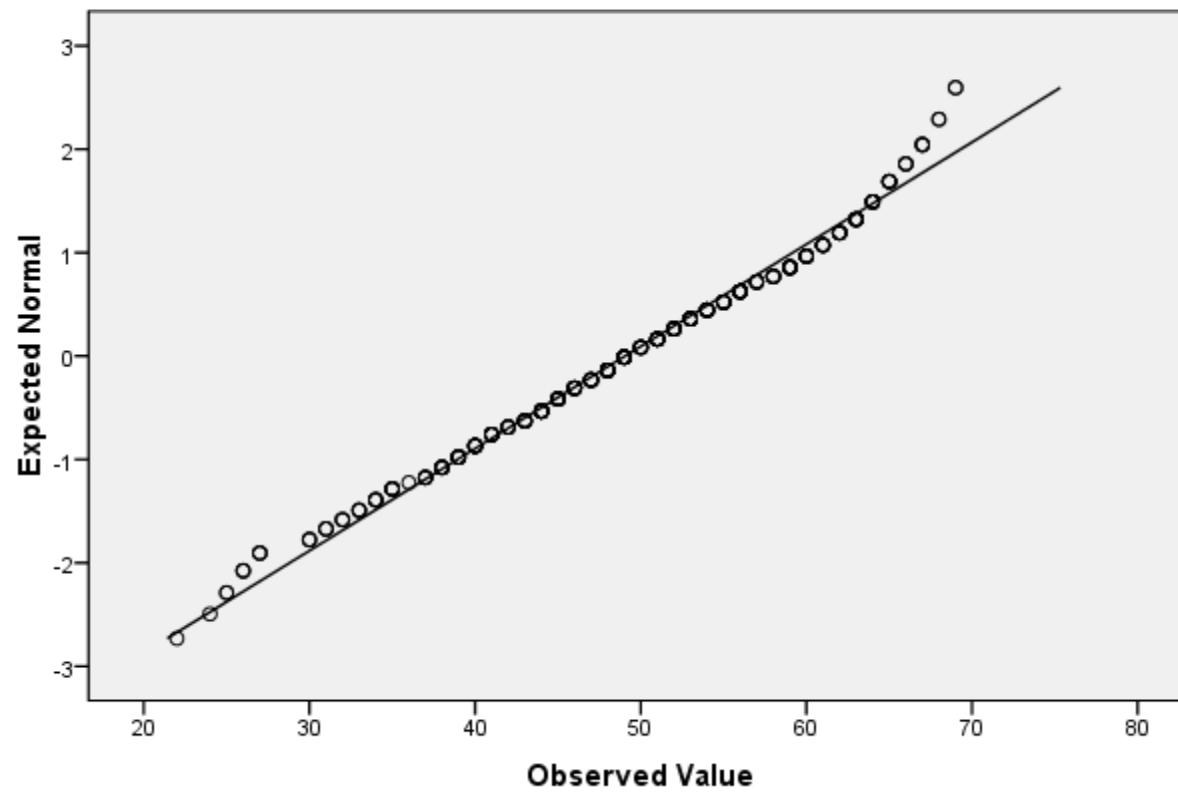
Normal Q-Q Plot of Regulasi Emosi
