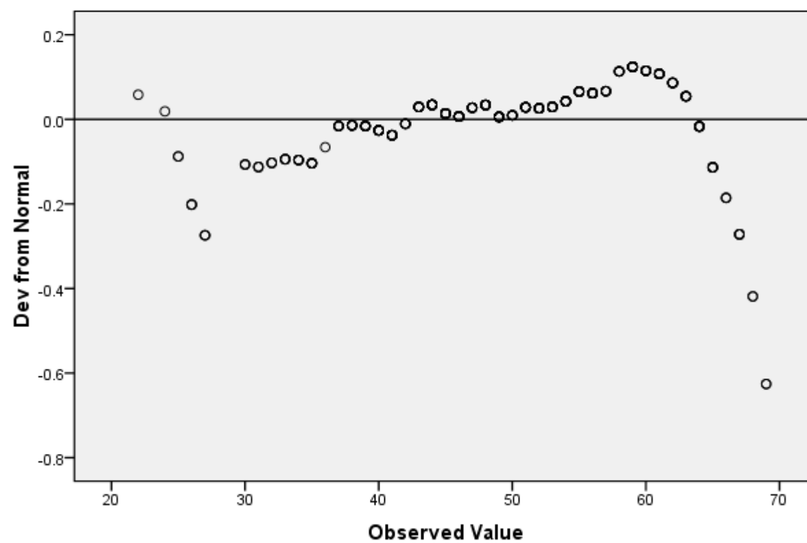
Detrended Normal Q-Q Plot of Regulasi Emosi
