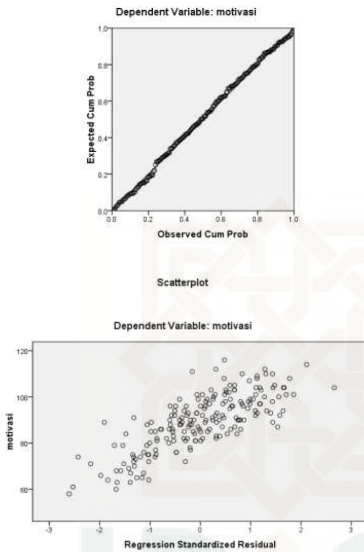
Normal P-P Plot of Regression Standardized Residual
