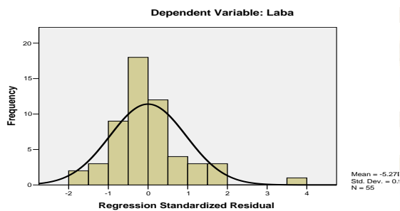
Histogram
