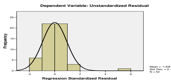
Histogram
