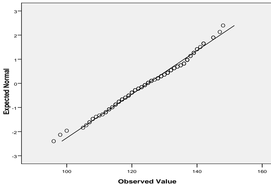
Normal Q-Q Plot of Disiplin Siswa
