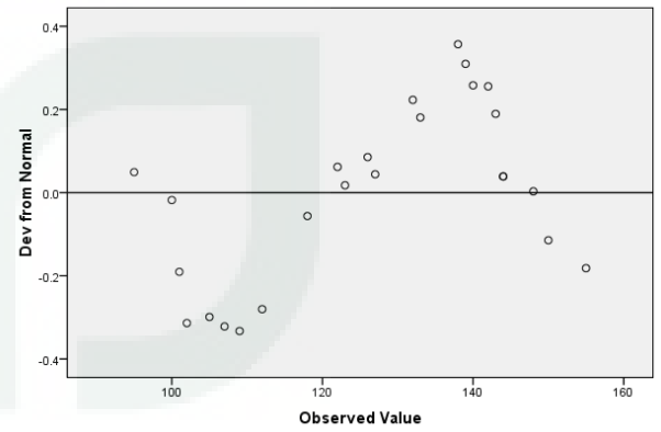
Detrended Normal Q-Q Plot of posttest
