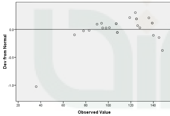
Detrended Normal Q-Q Plot of pretest
