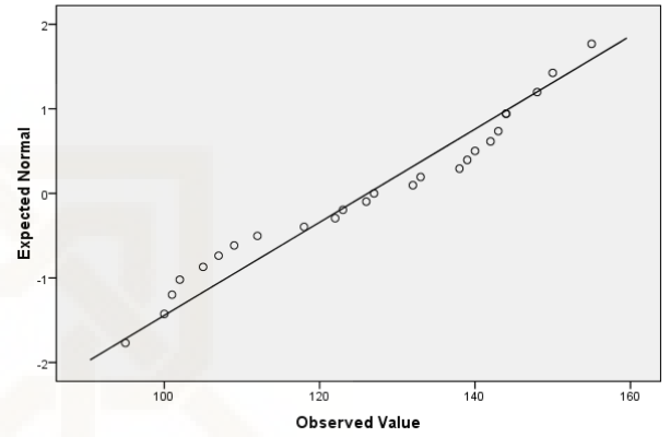
Normal Q-Q Plot of posttest
