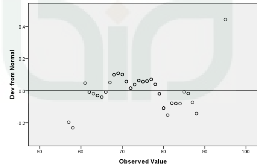
Detrended Normal Q-Q Plot of Kompetensi Interpersonal
