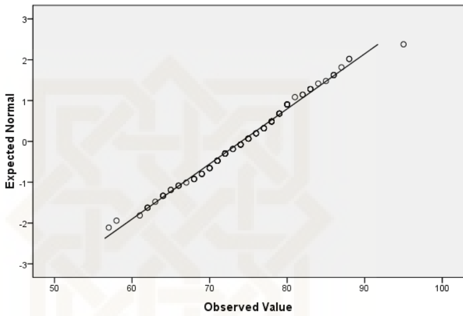
Normal Q-Q Plot of Kompetensi Interpersonal
