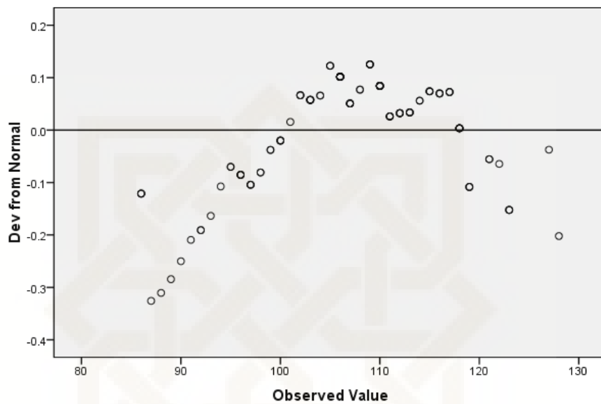
Detrended Normal Q-Q Plot of Dukungan Sosial
