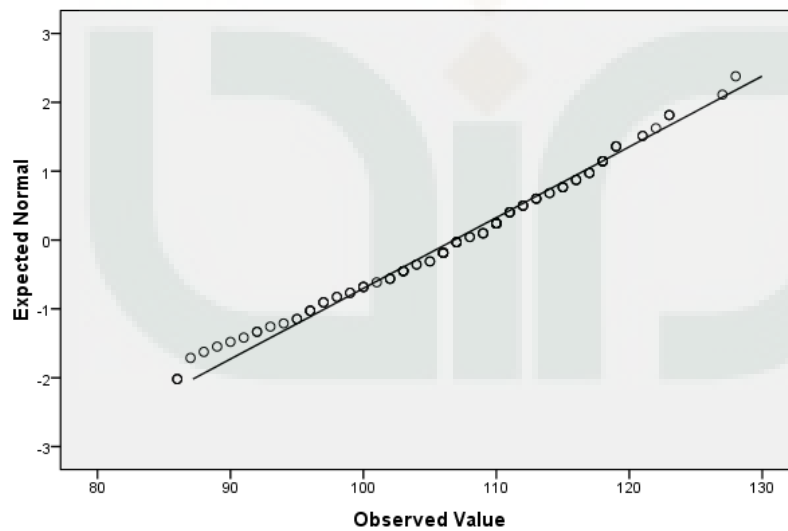
Normal Q-Q Plot of Dukungan Sosial
