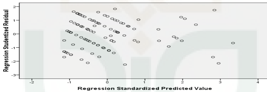
Scatterplot
