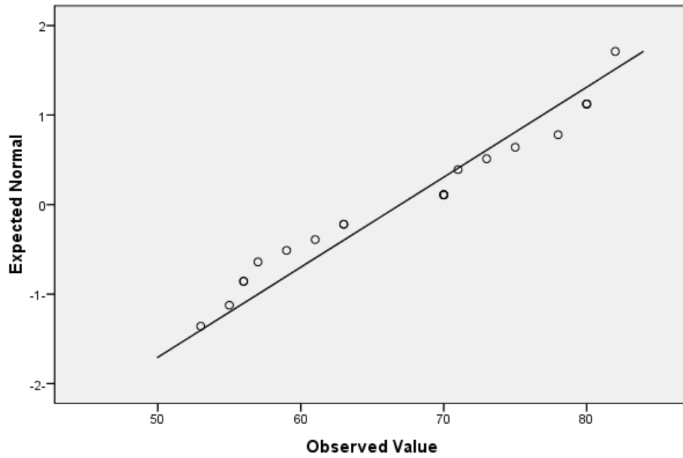
Normal Q-Q Plot of kalam_kontrol
