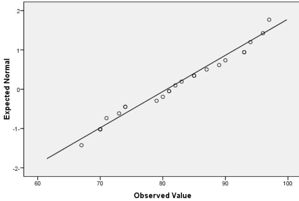
Normal Q-Q Plot of kalam_eks
