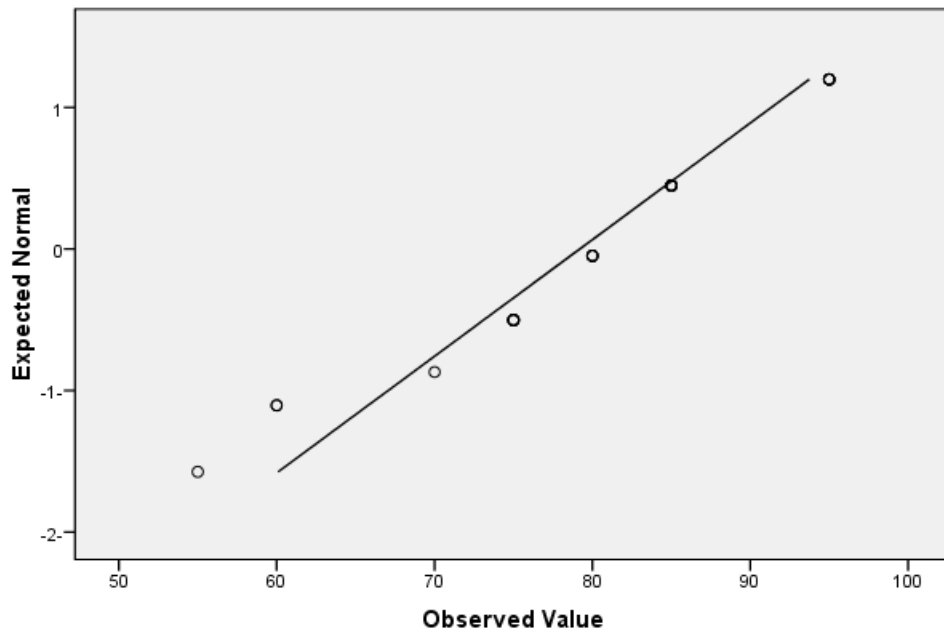
Normal Q-Q Plot of istima_eks
