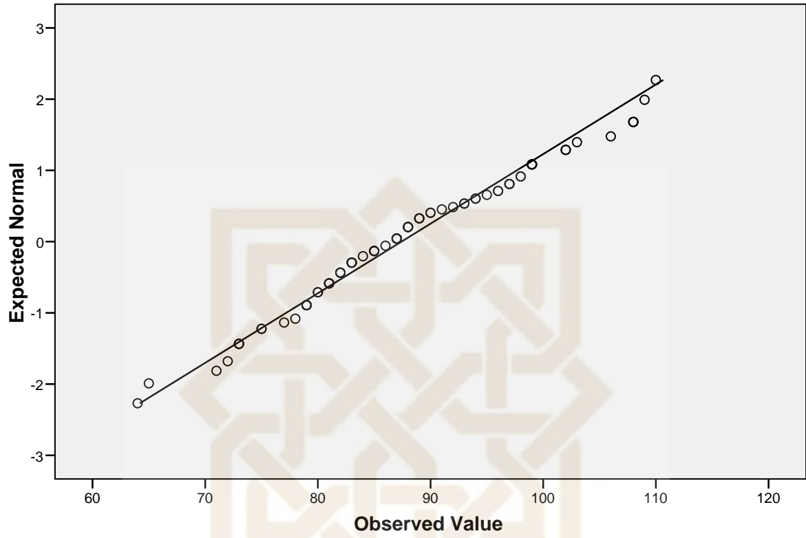
Normal Q-Q Plot of Layanan Informasi Karir
