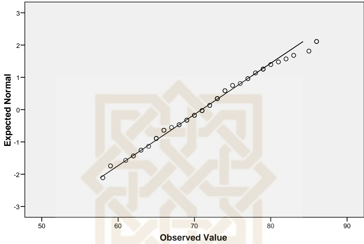
Normal Q-Q Plot of Minat siswa
