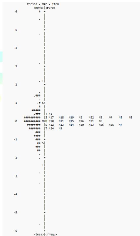
Figure 1 Item-person map
