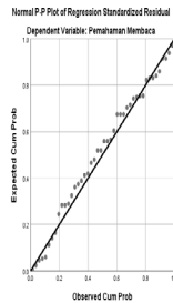
Gambar 1 Normal P-Plot
