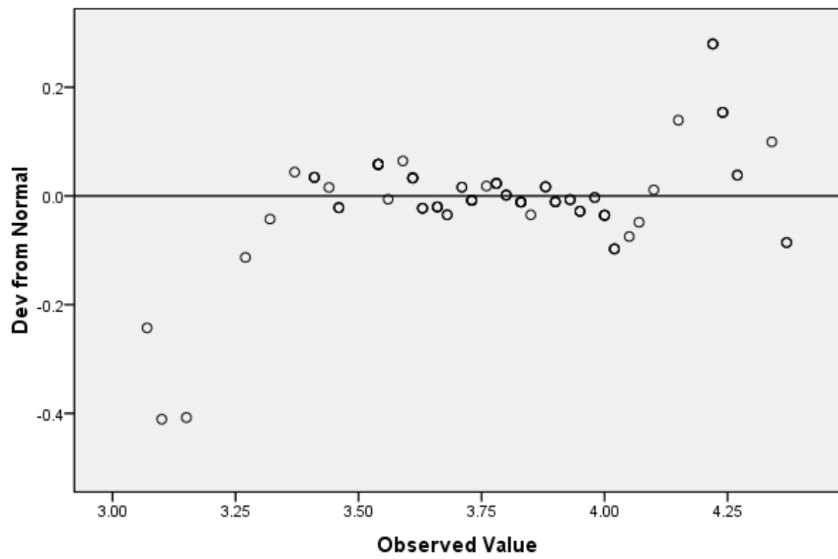
Detrended Normal Q-Q Plot of kedisiplinan siswa
