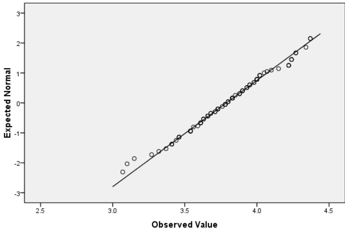
Normal Q-Q Plot of kedisiplinan siswa
