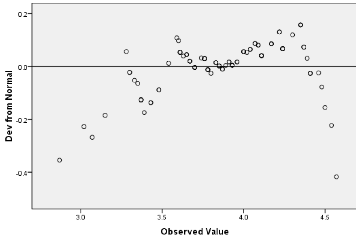
Detrended Normal Q-Q Plot of pembinaan keagamaan
